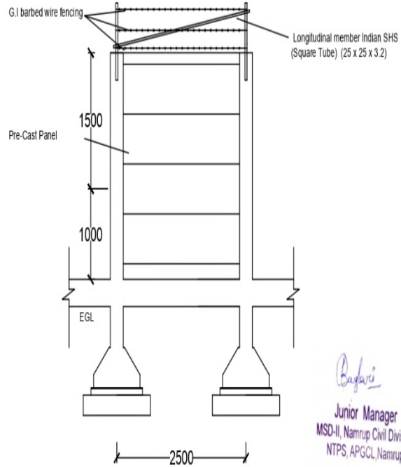
Elevation details of Boundary wall
