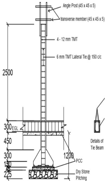
Sectional details of column at high level portion
