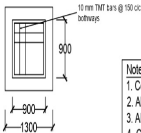
Foundation details of High & Low Level Portion
